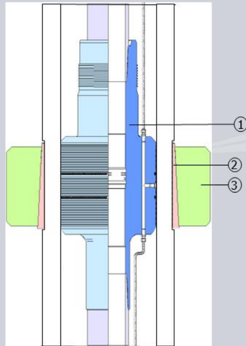
"HG" Hanger and Installation Tool
